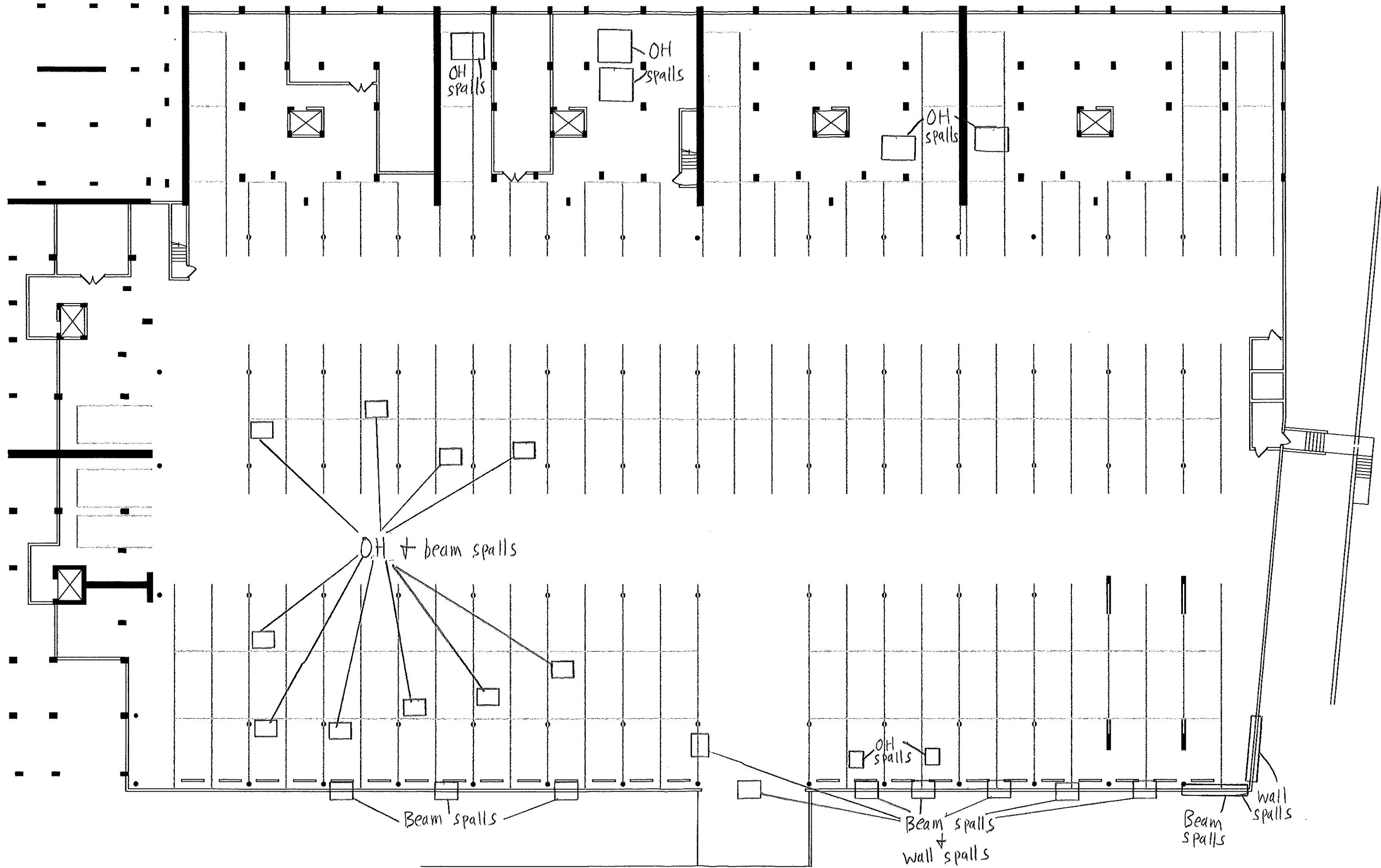
Plaza South BASEMENT LEVEL GARAGE PLAN (+10'-0") 1/16"=1'-0"
